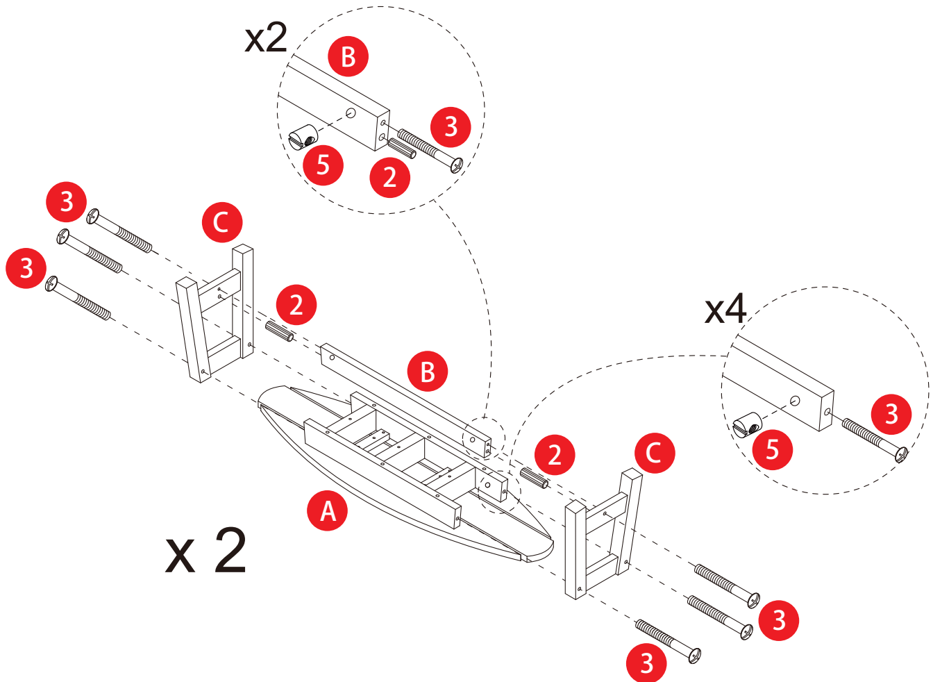
Assembled View: Stool
